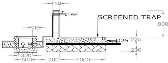
FRONT VIEW NTS
